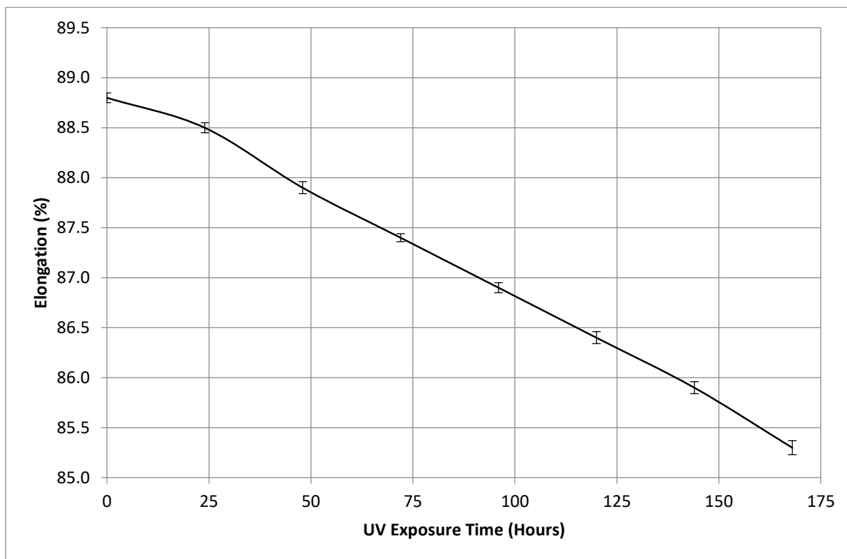
Figure 4: Elongation Versus UV Exposure Time (Hours)
