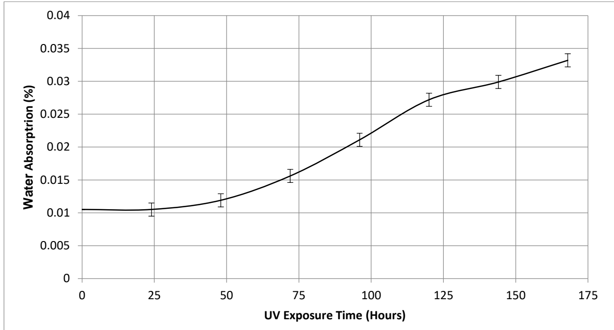
Figure 2: Water Absorption Versus UV Exposure Time (Hours)
