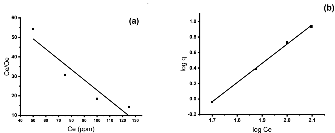
Figure 3. (a). Langmuir adsorption isotherm of MCPA sorption (adsorbent dose = 0.05g, contact time = 105 Minutes, initial concentration = 50 –150 mg L -1 , agitation speed = 120 rpm, T = 25±2 °C) ( R^2 = 0.995), (b). Freundlich adsorption isotherm of MCPA sorption (adsorbent dose = 0.05g, contact time = 105 Minutes, initial concentration = 50 –125 mg L -1 , agitation speed = 120 rpm, T = 25±2 °C) ( R^2 = 0.9987)
