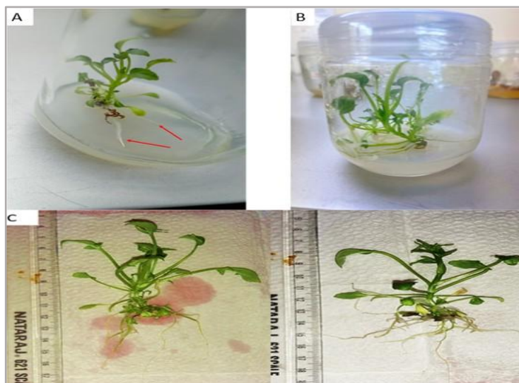
Figure 3. Root induction of in vitro shoots of V. moonii cultured on MS media supplemented with 2,4D 1.5mg/L and Kn 1.0mg/L. (a)Roots emerged from in vitro shoots after 17 days of inoculation. (b)Generated roots from in vitro shoots after 4 weeks of inoculation. (c)Plantlets of V.moonii removed from root induction culture medium after 5 weeks of inoculation.
