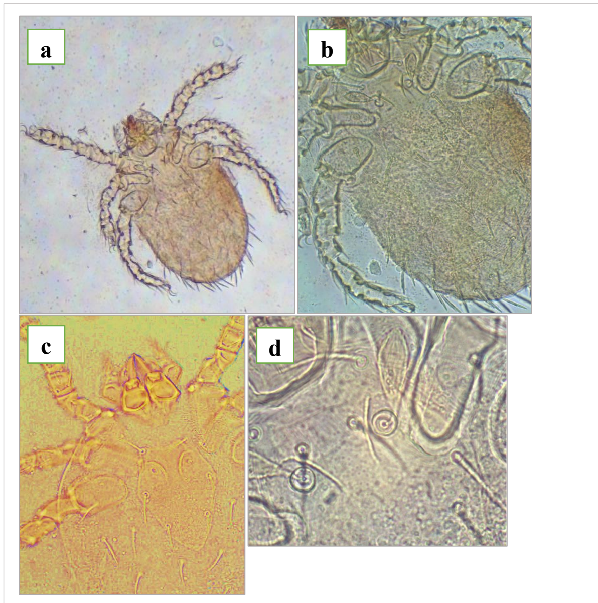
Figure 4. Microscopic view of Schoengastiella punctata (a) whole mount (10 x 20), (b) Whole mount (10 x 40), (c) Elongated scutum (10 x 60), (d) Scutum- sensila (10 x 100)
