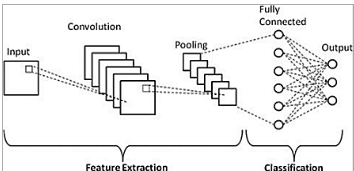
Figure 4. CNN Architecture
