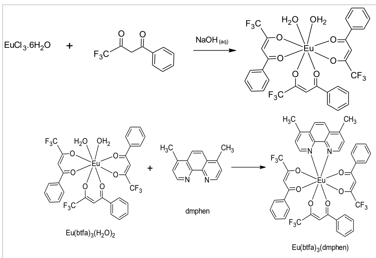
Figure 1. Synthesis of \text{Eu}(\text{btfa})_3(\text{dmphen}) complex
